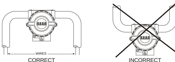
Figure 1.6 - Conduit Installation
