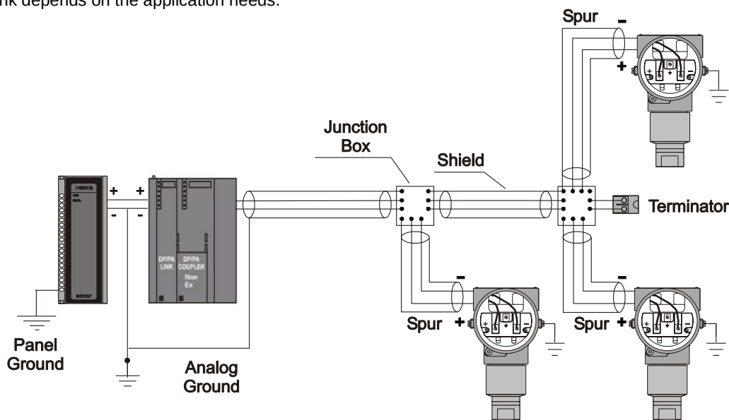
Figure 1.8 - Bus Topology
