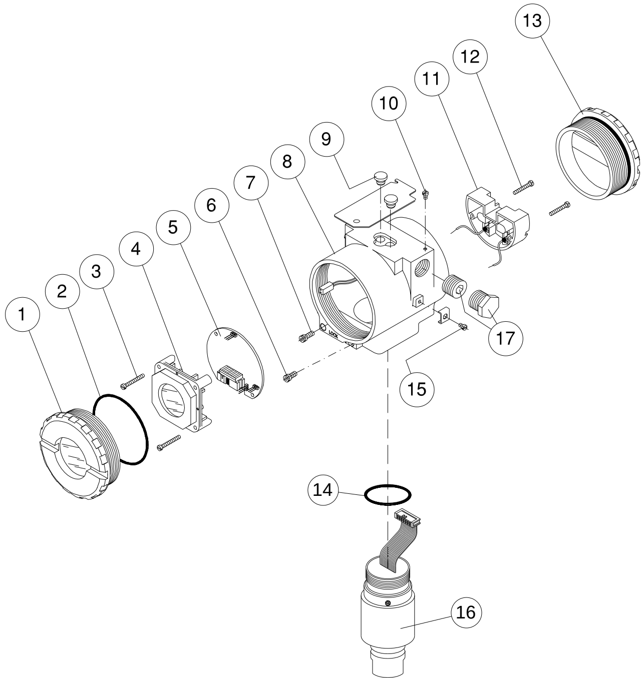
Figure 4.3 – Exploded View
